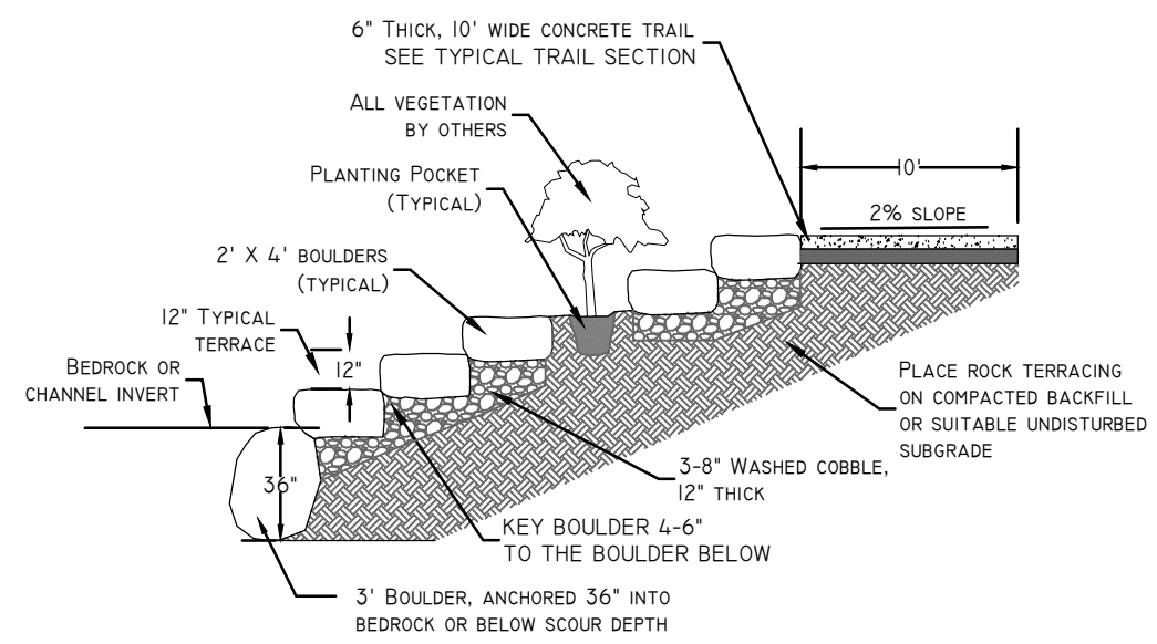
TERRACED ROCK WITH PLANTING POCKET TYPICAL N.T.S
